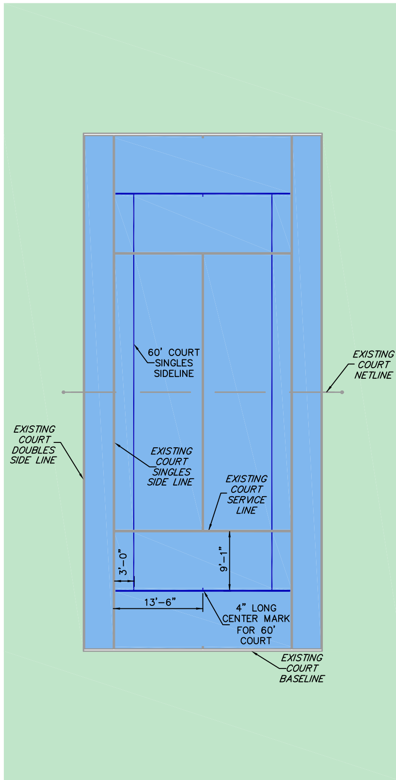
SHARED LINES ON A 78 FOOT COURT NOT TO SCALE
