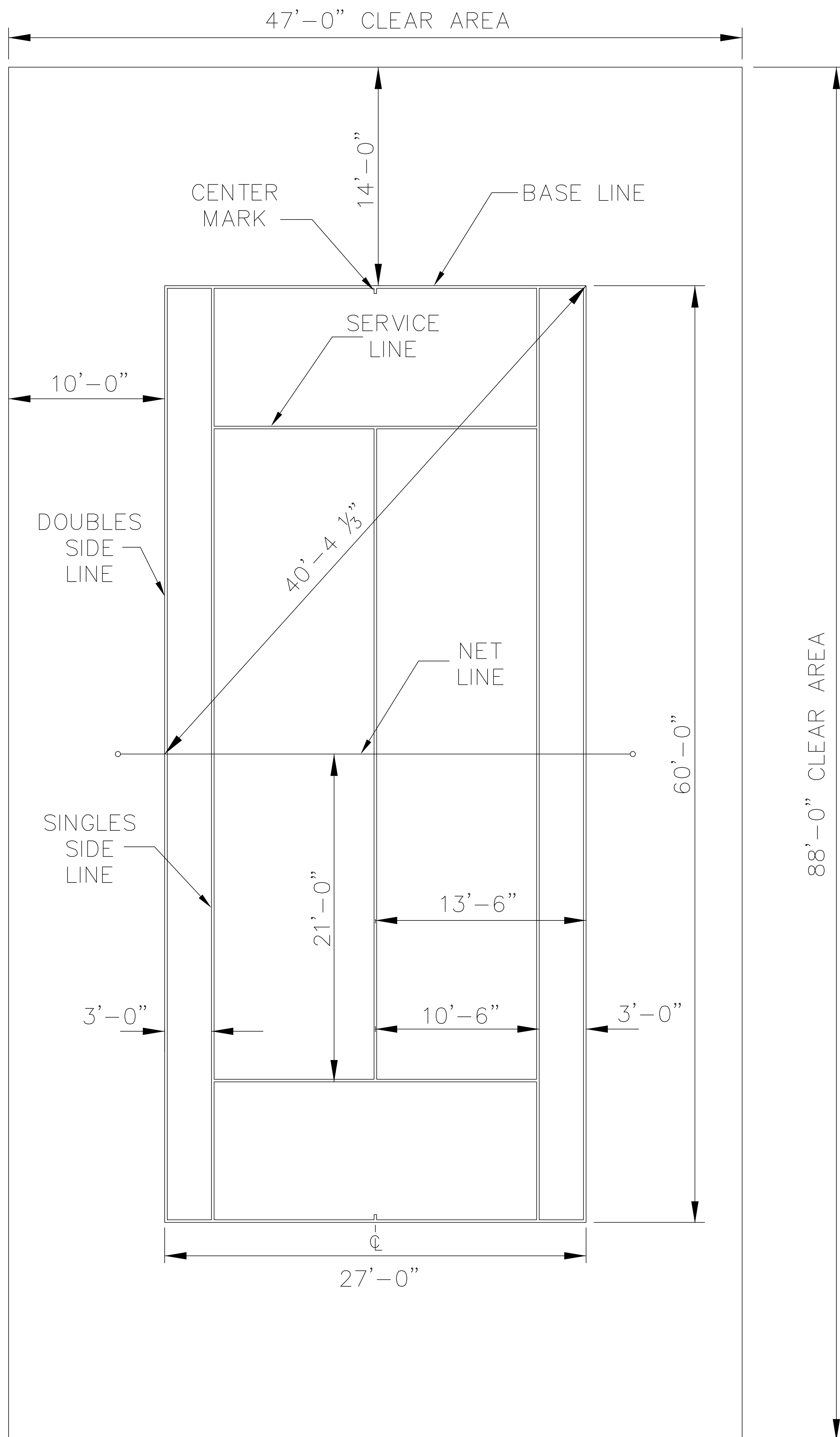
SINGLE COURT LINE LAYOUT NOT TO SCALE
